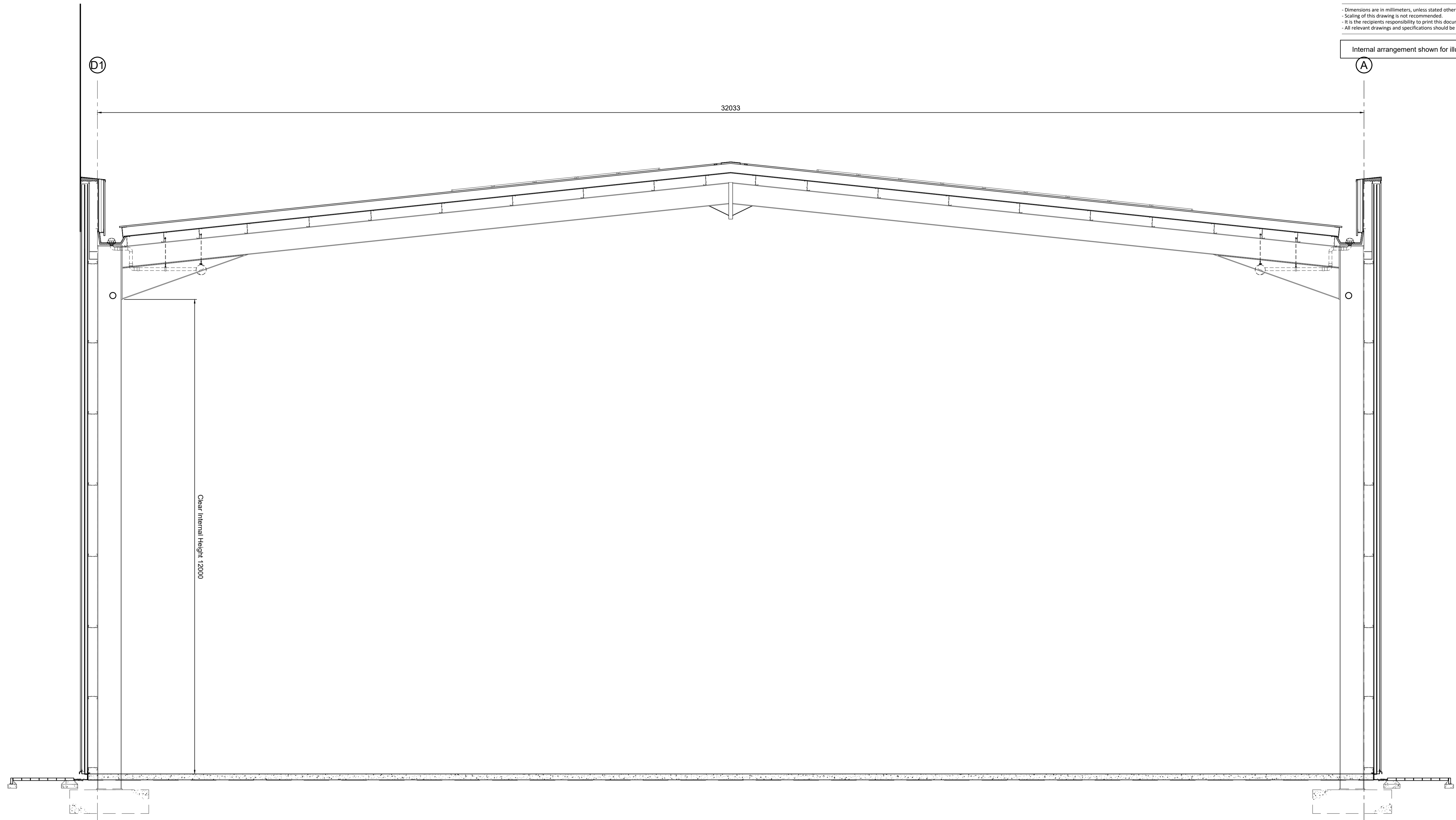
Cross Section Scale 1:50
