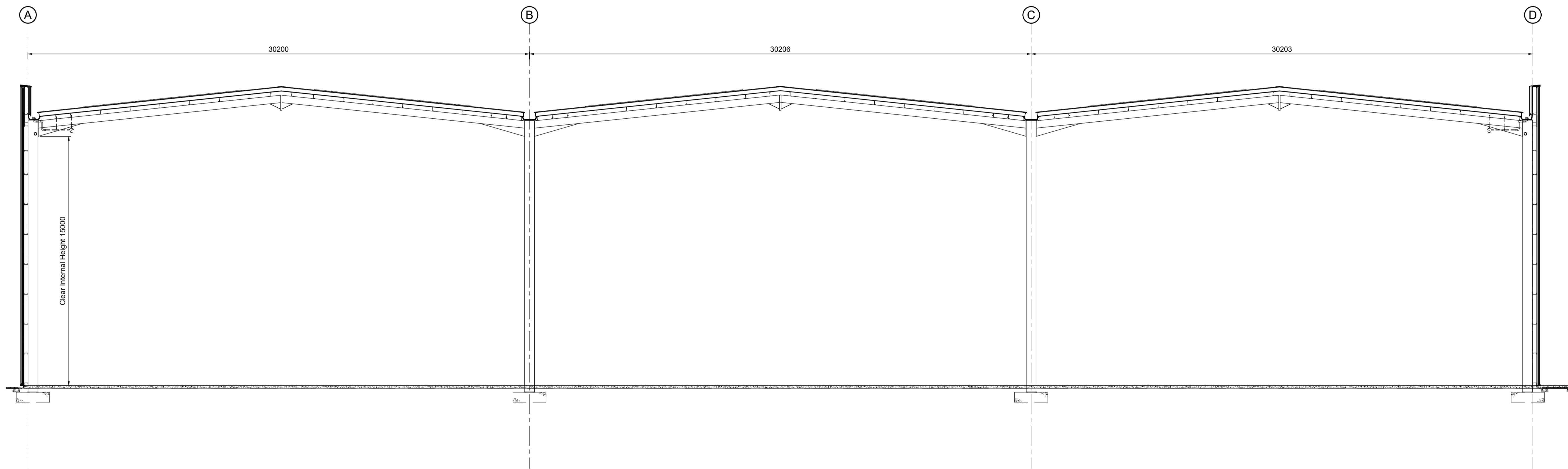
Cross Section Scale 1:125
